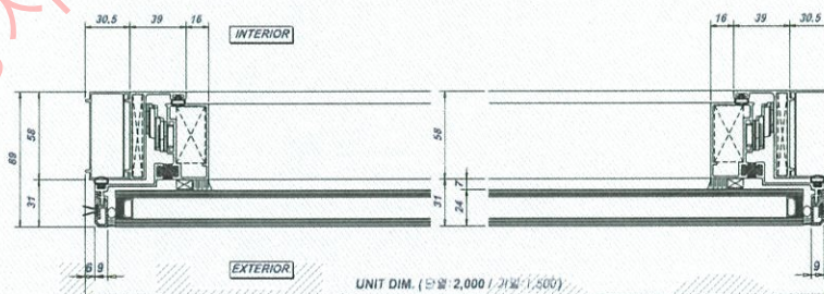
HORIZONTAL SECTION DETAIL B-B'
