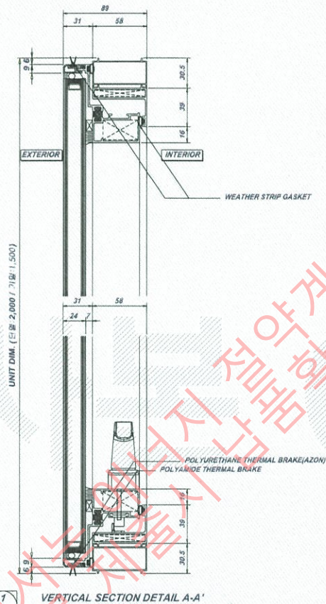
VERTICAL SECTION DETAIL A-A'
